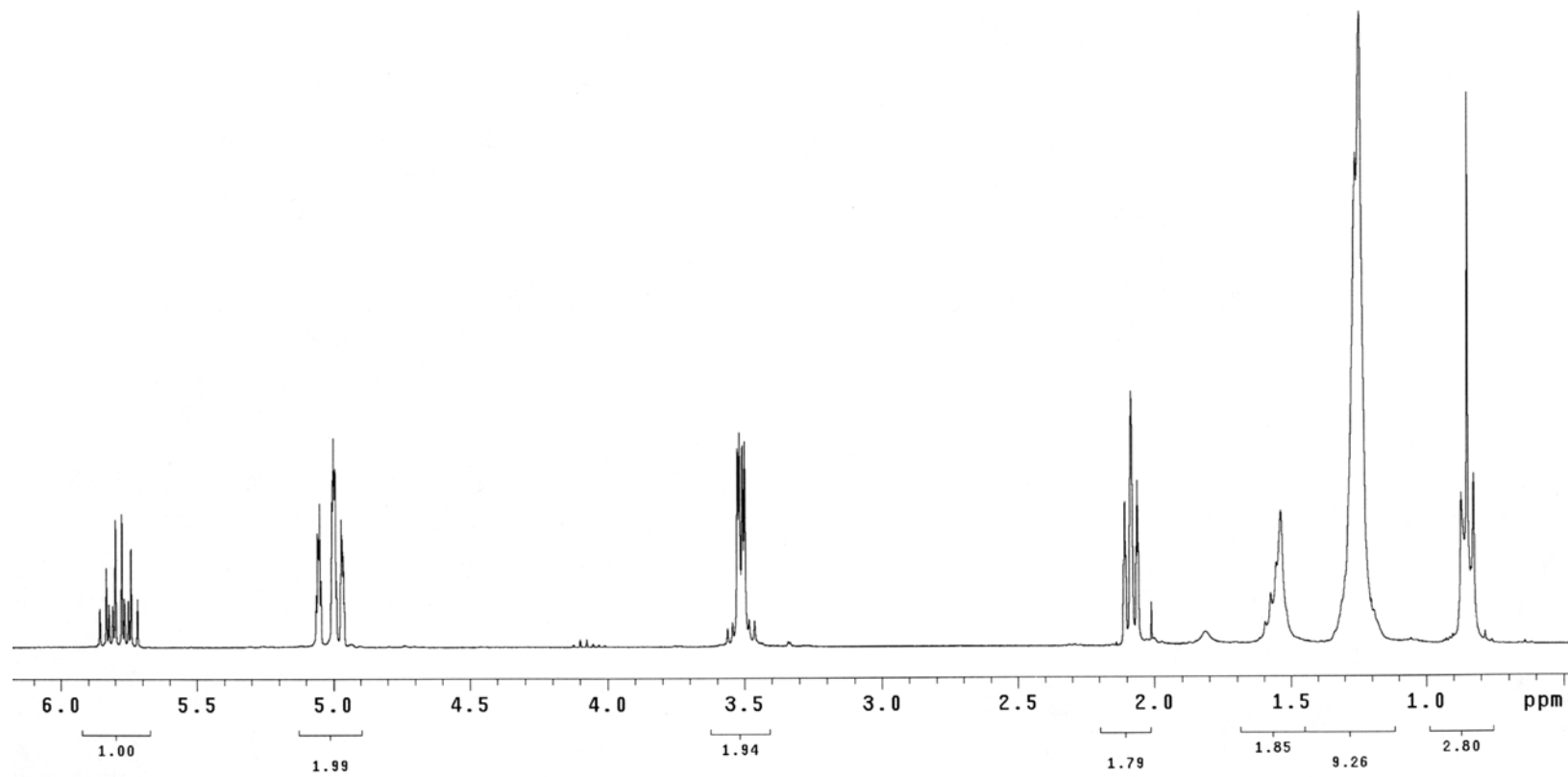
Figure 7. ^1\text{H} NMR Spectrum of 8 in \text{CDCl}_3 (300 MHz)
