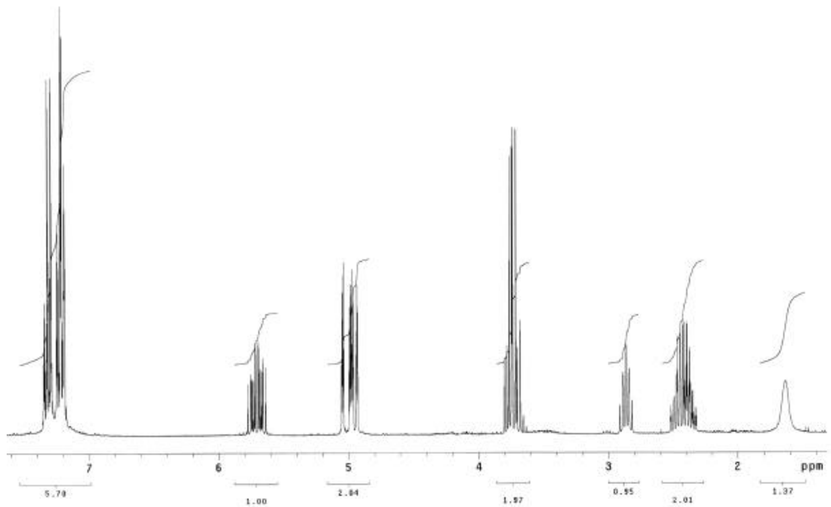
Figure 2. ^1\text{H} NMR Spectrum of 3 in \text{CDCl}_3 (300 MHz)
