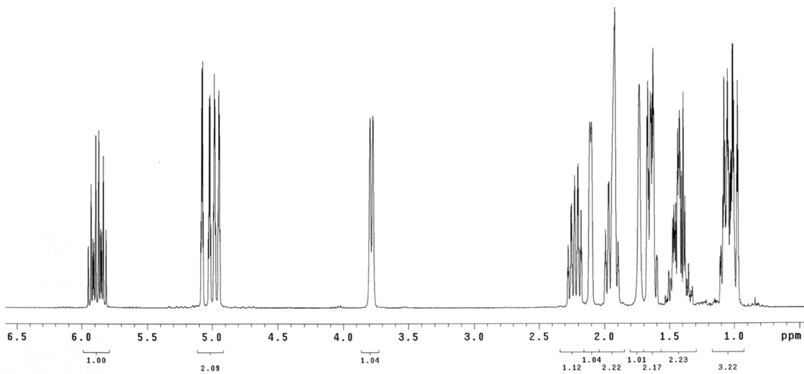
Figure 3. ^1\text{H} NMR Spectrum of 4 in \text{CDCl}_3 (300 Mhz)
