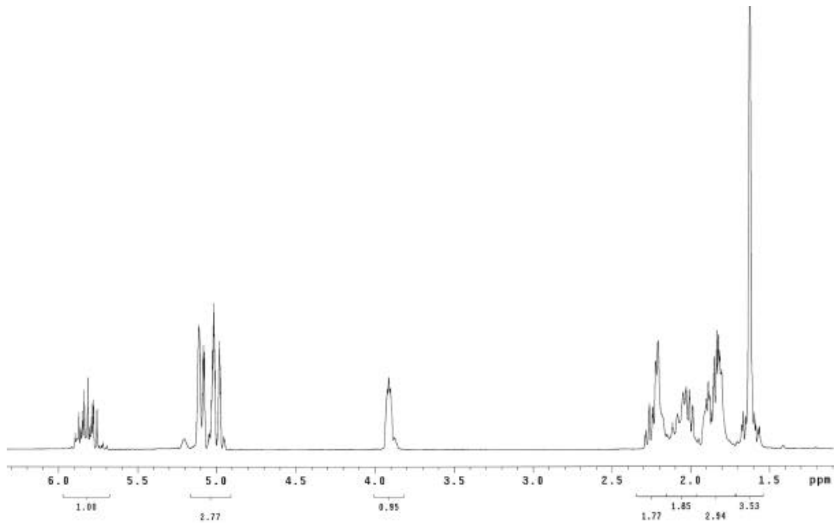
Figure 5. ^1\text{H} NMR Spectrum of 6 in \text{CDCl}_3 (300 Mhz). See note about impurity above.
