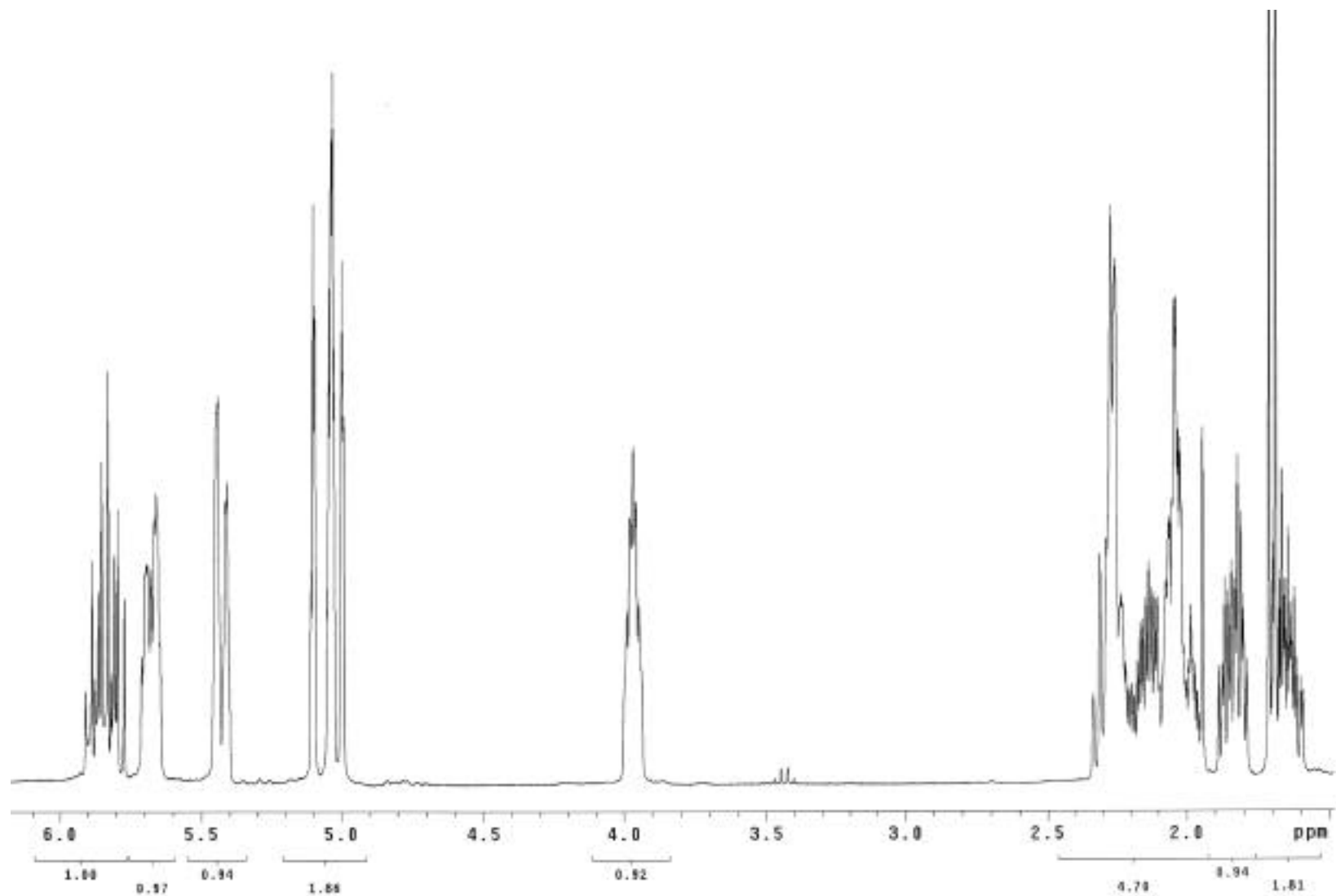
Figure 1. ^1\text{H} NMR Spectrum of 2 in \text{CDCl}_3 (300 MHz)
