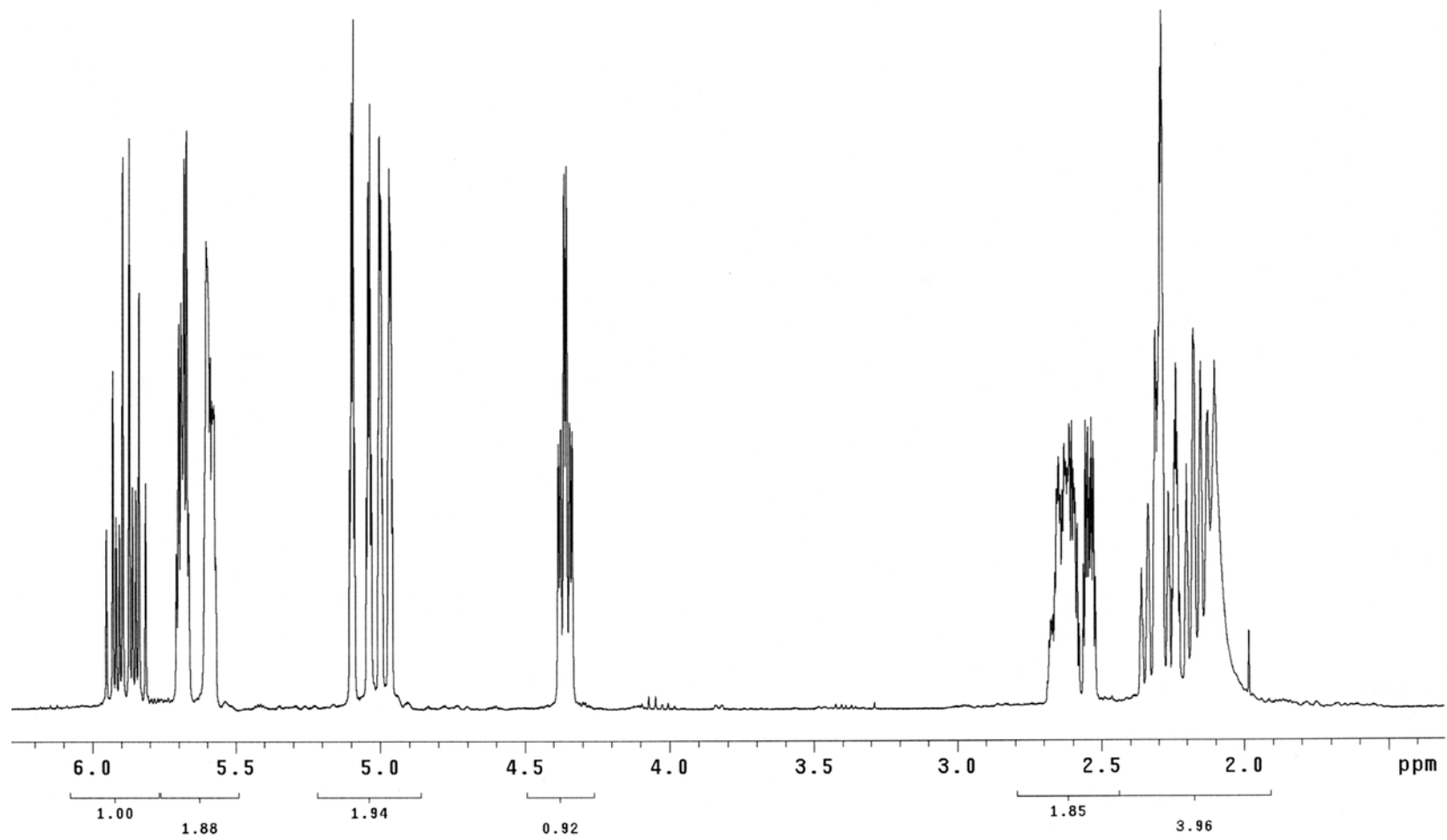
Figure 6. ^1\text{H} NMR Spectrum of 7 in \text{CDCl}_3 (300 MHz)
